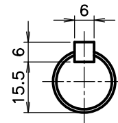
OUTPUT SHAFT
