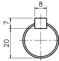
OUTPUT SHAFT
