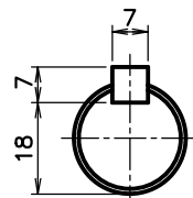
OUTPUT SHAFT
