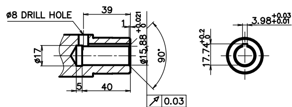
OUTPUT SHAFT
