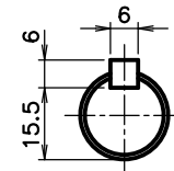
OUTPUT SHAFT
