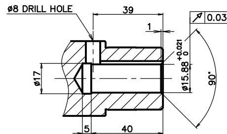
OUTPUT SHAFT
