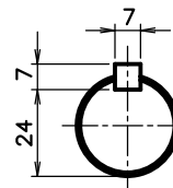
OUTPUT SHAFT
