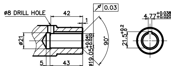
OUTPUT SHAFT
