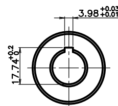
OUTPUT SHAFT
