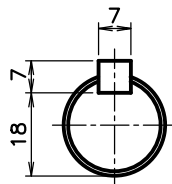
OUTPUT SHAFT
