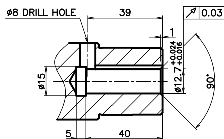
OUTPUT SHAFT
