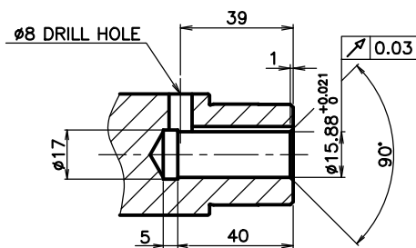
OUTPUT SHAFT
