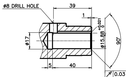
OUTPUT SHAFT
