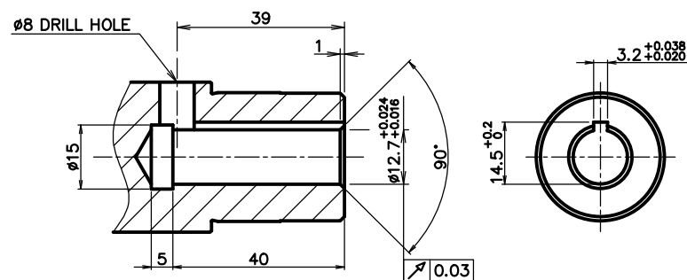
OUTPUT SHAFT
